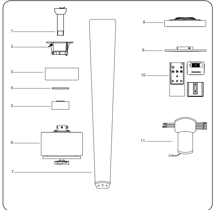
12 Loose part
